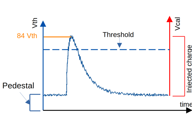
Figure 4.22: Injected charge plus pedestal for a specific channel.
