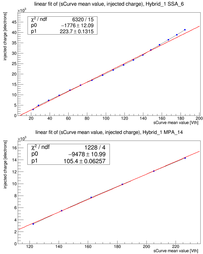
Figure 4.25: Conversion from Vth to electrons for Hybrid 1, SSA 6 (strips) and MPA 14 (pixels)
