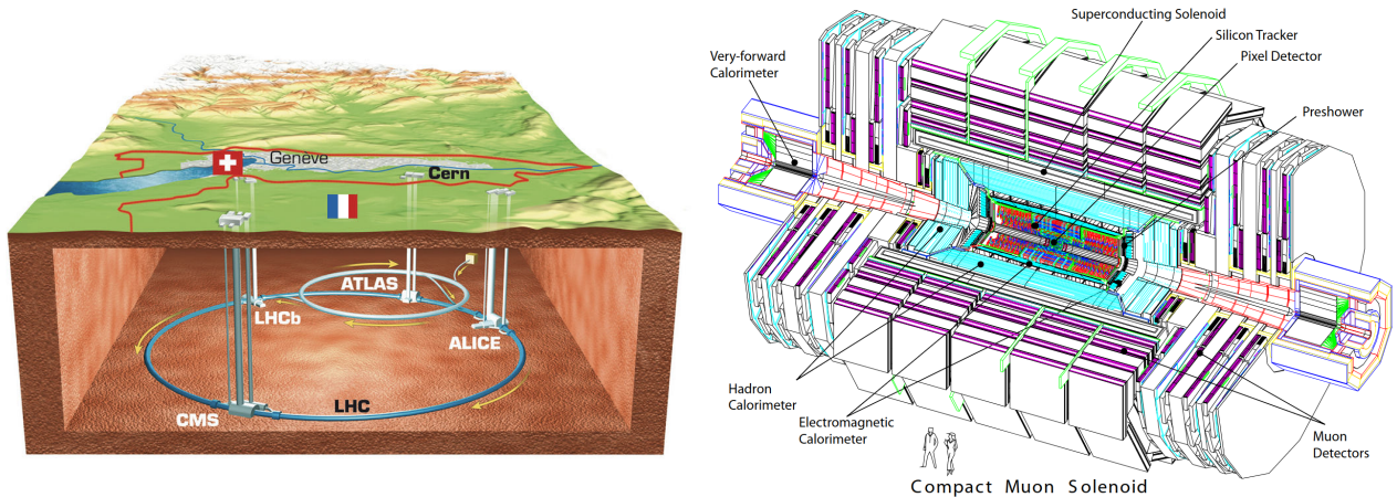
Figure 1.1: on the left a brief scheme of LHC, on the right one for the CMS experiment.
